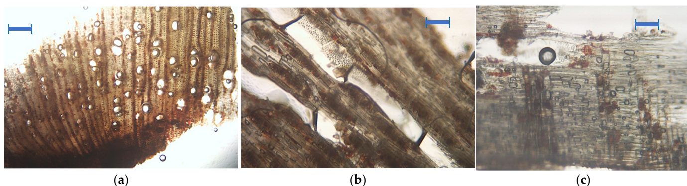
Figure 2. Microscopy observation of the thin wood sections, three anatomical directions: (a) transverse; (b) tangential; (c) radial. The bars correspond to 100 µm.
